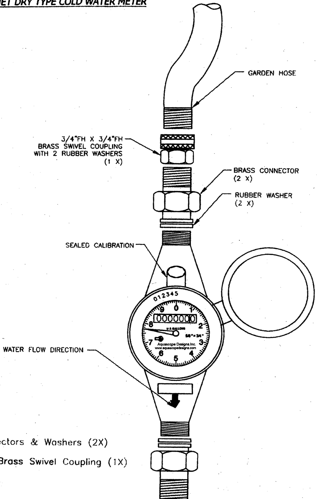
CONNECTING SCHEMATIC
